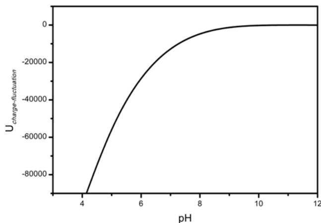
Fig. 2. Charge fluctuation contribution to the interaction energy as a function of solution pH: I=0.03 M, H/kT=8.9 , \Delta r=0.8 Å, \epsilon/kT=4.5 Å, \delta=4 Å, d_s=0.694 Å, d_{11}=3.5 nm, d_{22}=3.4 nm.
